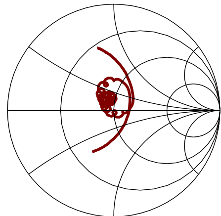
S22 (220-260 MHz)
