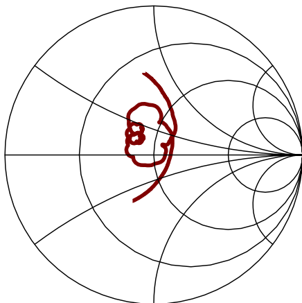
S11 (220-260 MHz)
