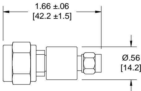
Model Number: 5015 TNC Male / SMA Male
