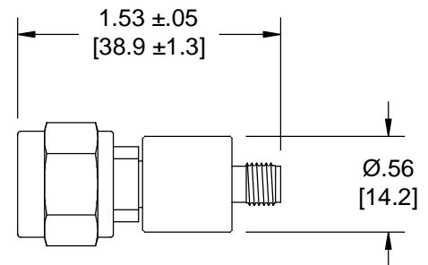
Model Number: 5017 TNC Male / SMA Female
