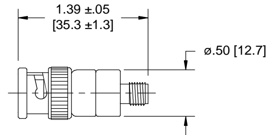
Model Number: 5013 BNC Male / SMA Female
