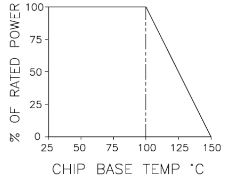
AVERAGE POWER DERATING
