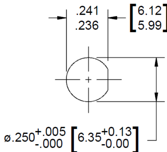
Recommended Mounting Hole
