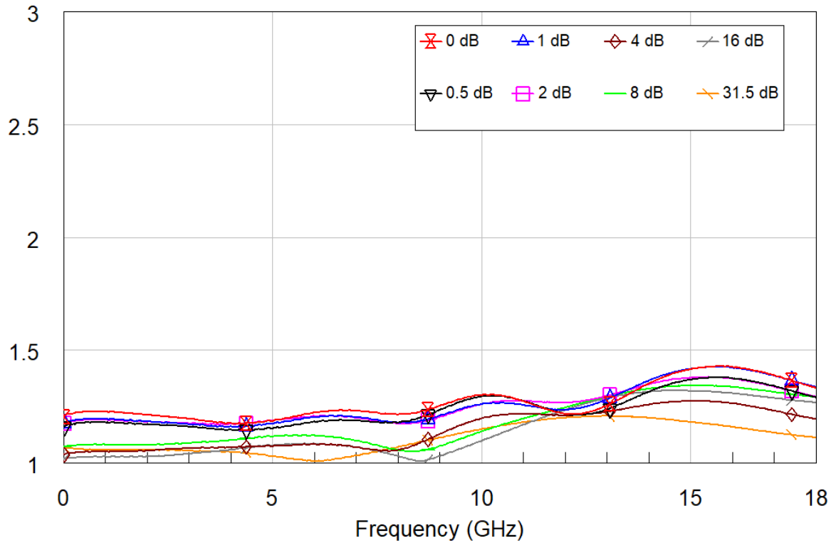
VSWR at Port J2
