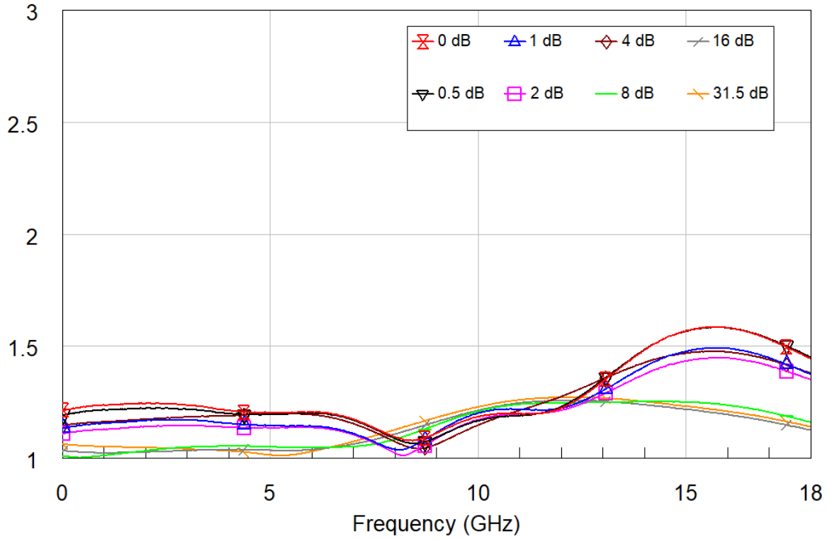
VSWR at Port J1
